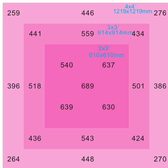
FM8 660W 2.4µmol/J 24''/609mm Height
